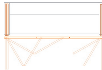
REVEGO duo + uno For widths of 1350 – 2400 mm
